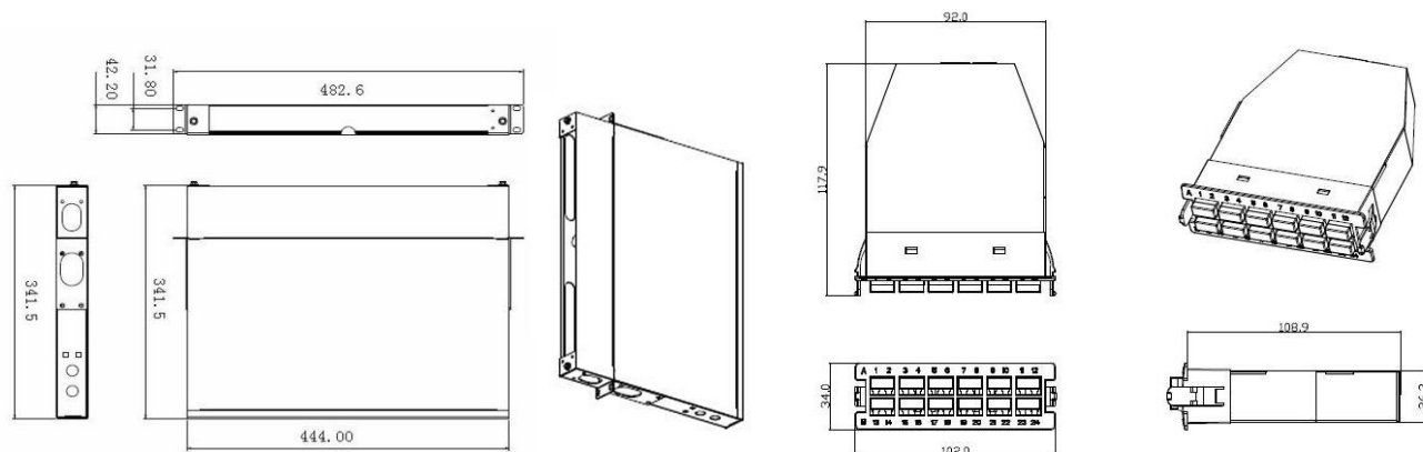
Racks: TK-HRF-1096A
